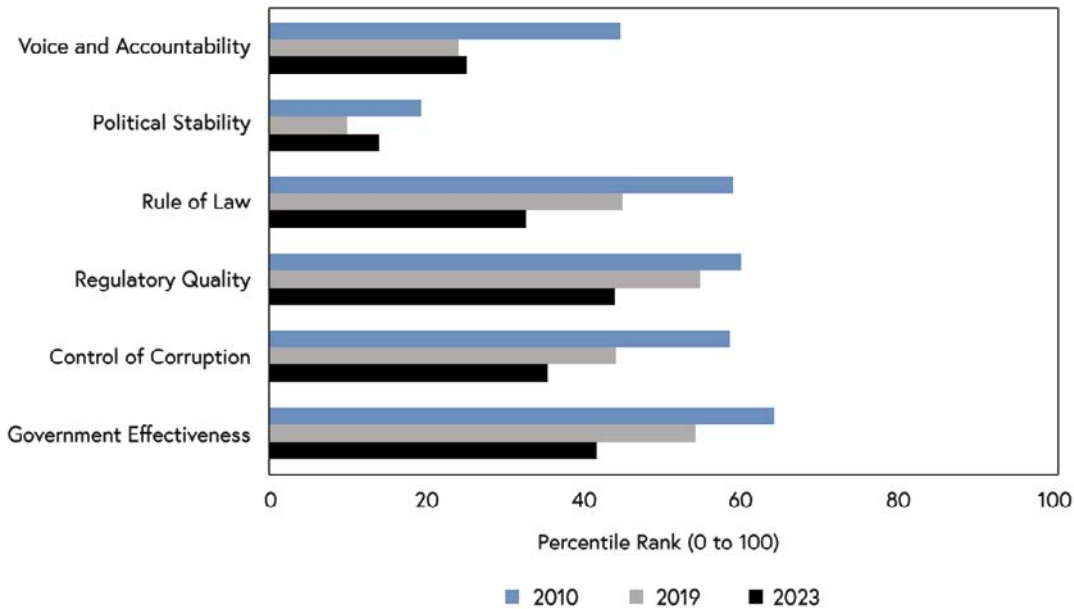
Chart 2: Country's Worldwide Governance Indicators have deteriorated over time
